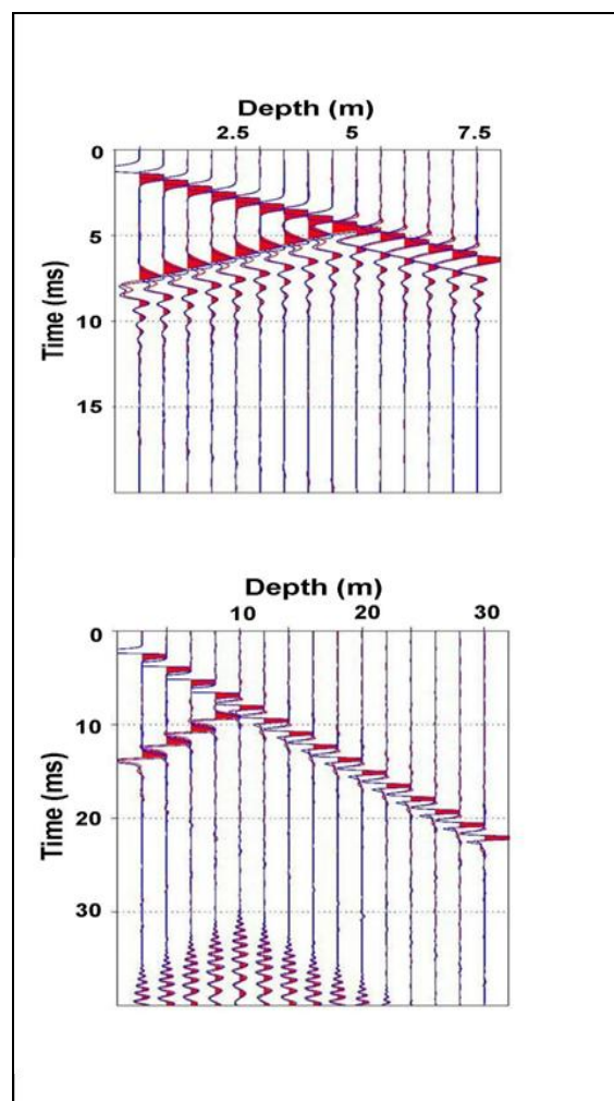
Figure 3. Wavefield in a borehole intersected by a fracture: (a) fracture 0.36 m; (b) fracture 10 m.
