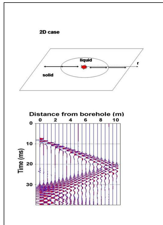
Figure 2. (a) 2D model used for deriving reflection coefficient from the tip. (b) Wavefield inside the fracture with length 10 m.
