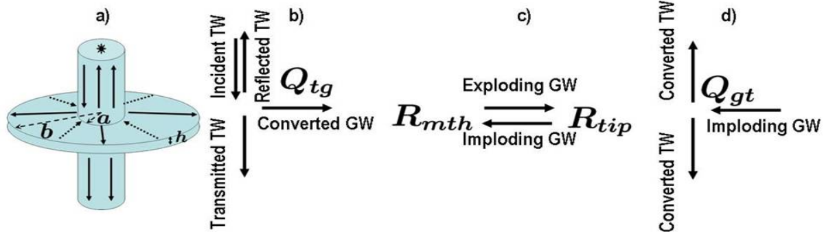
Figure 1. (a) Model geometry. (b)–(d) Simple representation of the wave propagation sequence.
