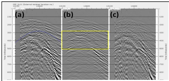
Figure 4: Receiver line from a 3D common-shot gather at different processing stages: (a) raw data, (b) after 3D FK filtering, and (c) difference between (a) and (b), highlighting the removed noise.
