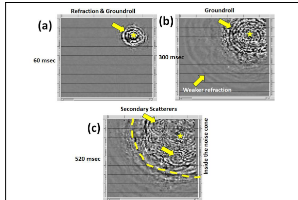
Figure 5: Time slices from the full receiver carpet for a single shot at the NW corner at different time positions—(a) 60 ms, (b) 300 ms, and (c) 520 ms—illustrating wavefield evolution in the raw data.
